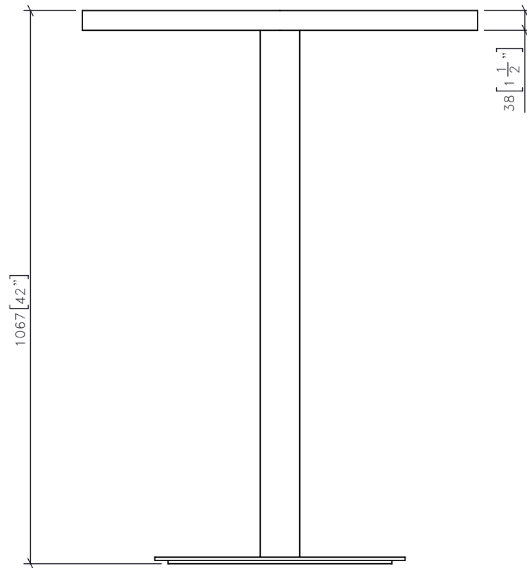
1 CG-16 HIGH TOP TABLE FRONT ELEVATION 1:10
