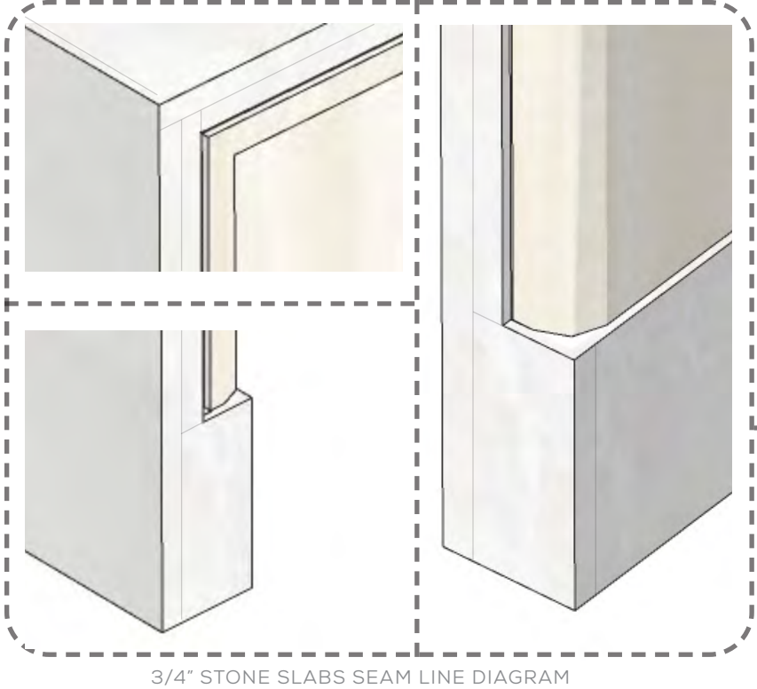
3/4" STONE SLABS SEAM LINE DIAGRAM
