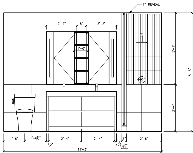
9 ID4.1 | LEVEL 12_BATHROOM 1/2"=1' | ELEVATION
