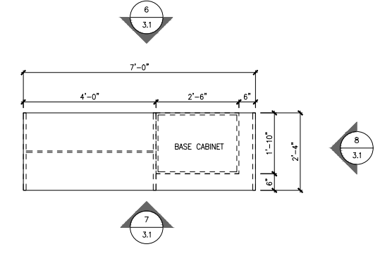
5 ID3.1 | LEVEL 12_KITCHEN OPT 2 ISLAND ENLARGED PLAN 1/2"=1'
