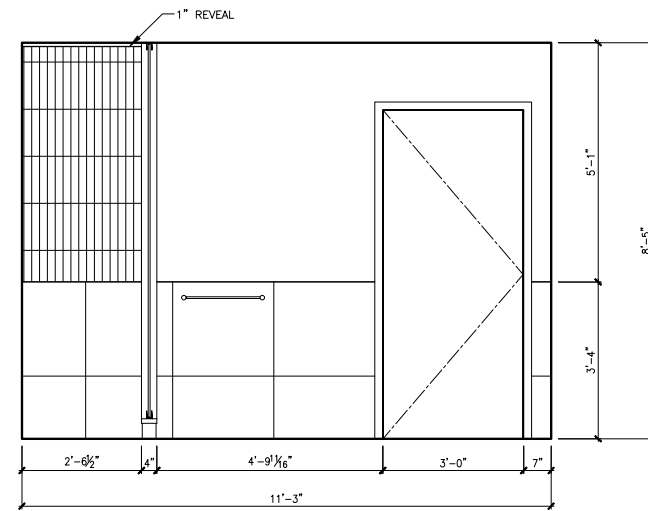
7 ID4.1 | LEVEL 12_BATHROOM 1/2"=1' | ELEVATION
