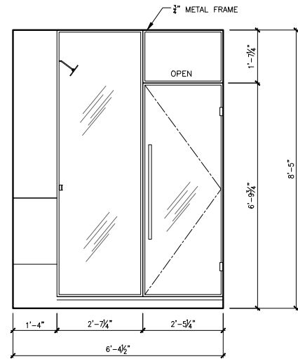
8 ID4.1 | LEVEL 12_BATHROOM 1/2"=1' | ELEVATION
