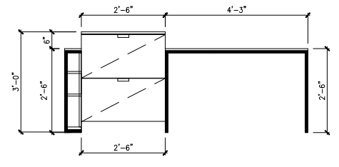
6 ID3.1 | LEVEL 12_KITCHEN OPT 2 ISLAND ELEVATION 1/2"=1'
