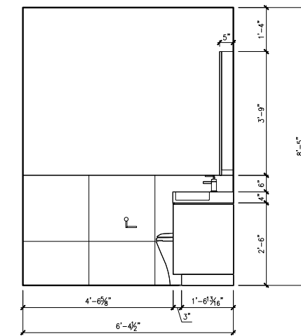
6 ID4.1 | LEVEL 12_BATHROOM 1/2"=1' | ELEVATION
