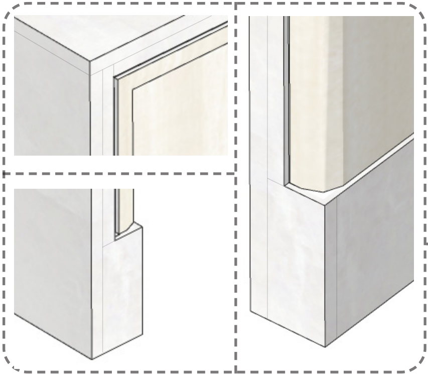
3/4" STONE SLABS SEAM LINE DIAGRAM
