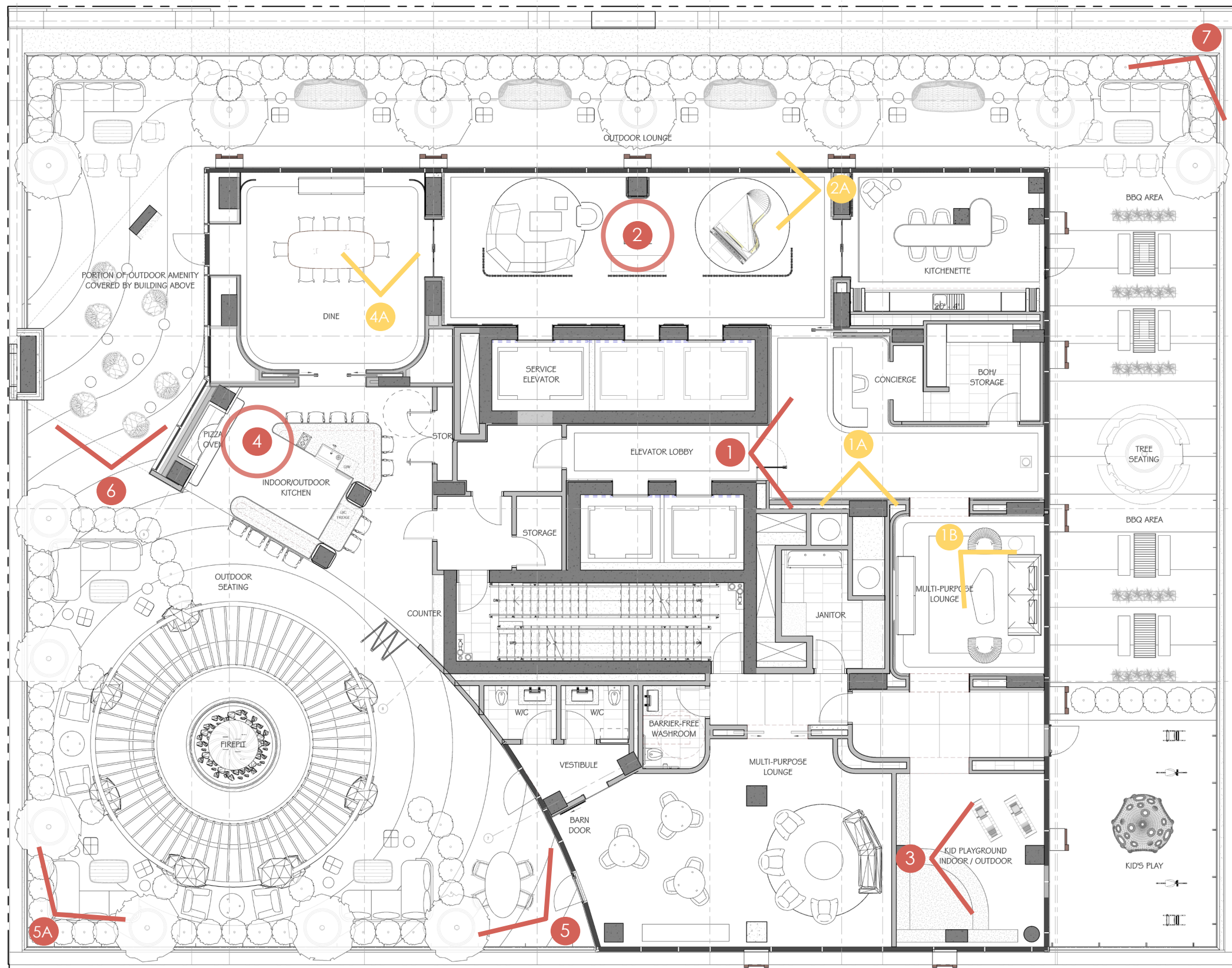
LEVEL 06 AMENITIES PLAN
