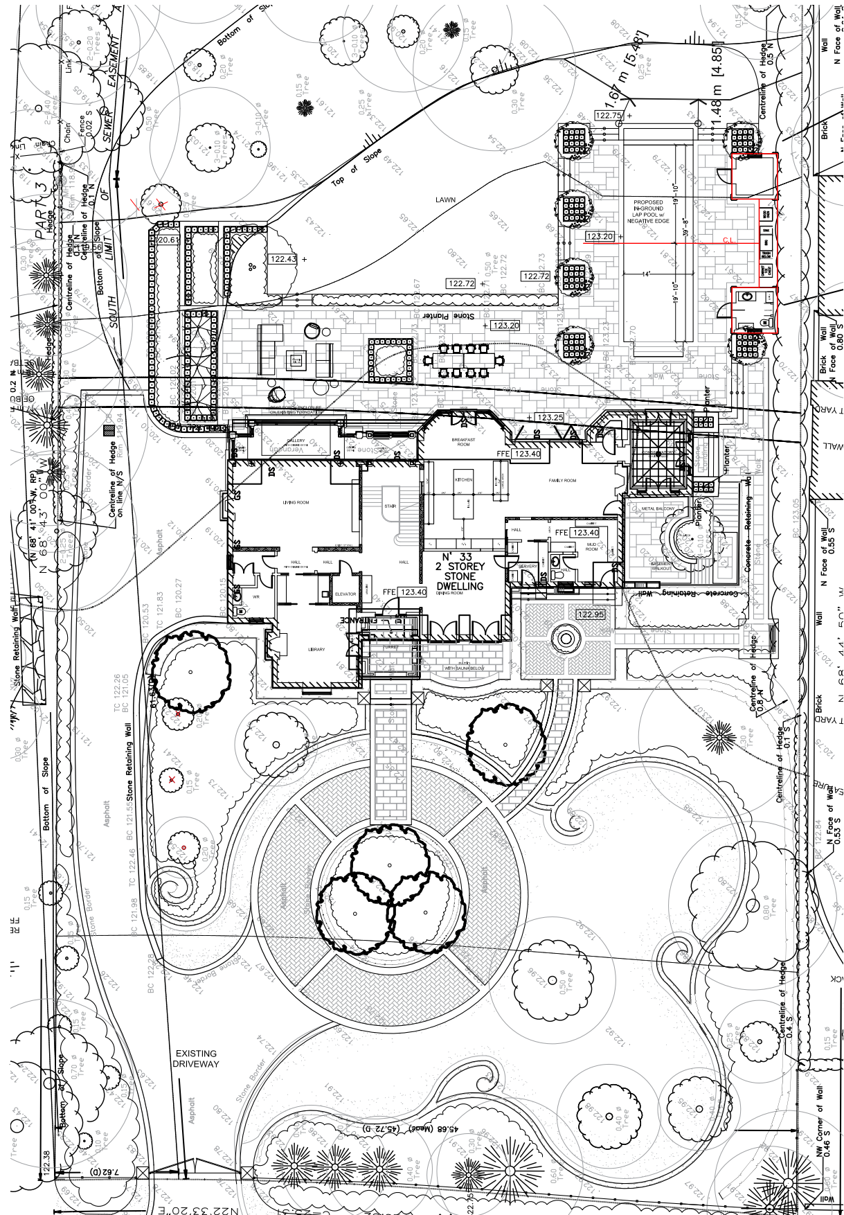
'BEFOR' LAYOUT
