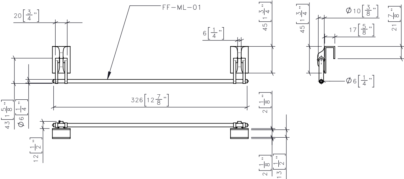
12 CG-310 MINIBAR 1:16 CUSTOM DRAWER PULL
