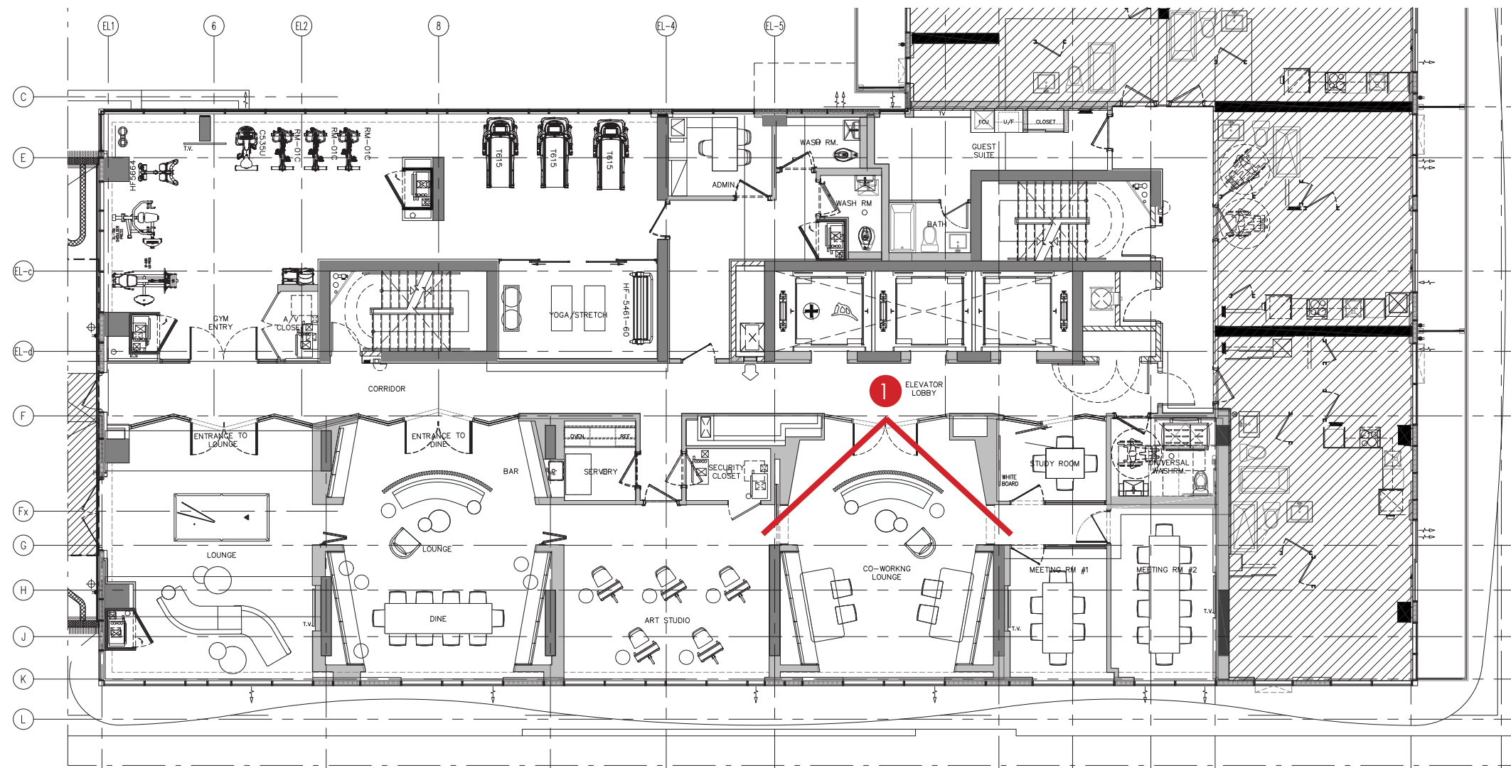
LEVEL 11 PLAN
