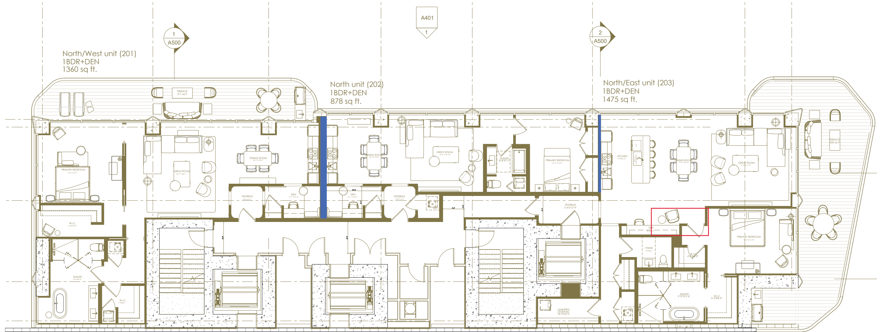
3rd FLOOR 3 UNIT PLATE STUDY
