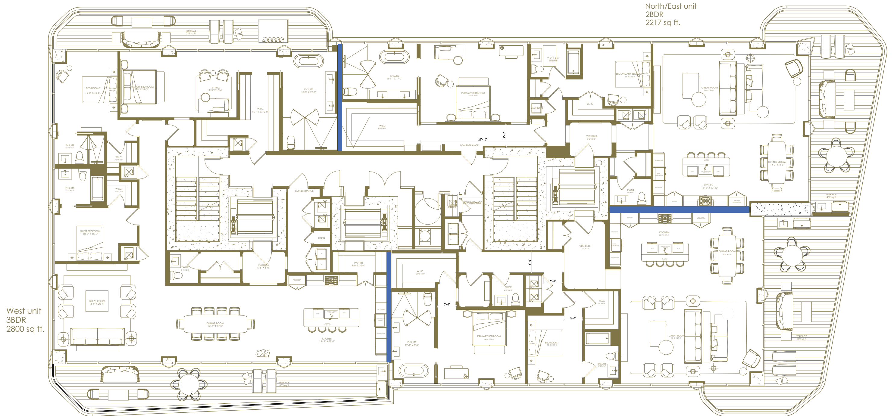
3 UNIT FLOOR PLATE STUDY SCALE: 1/4" = 1'-0"
