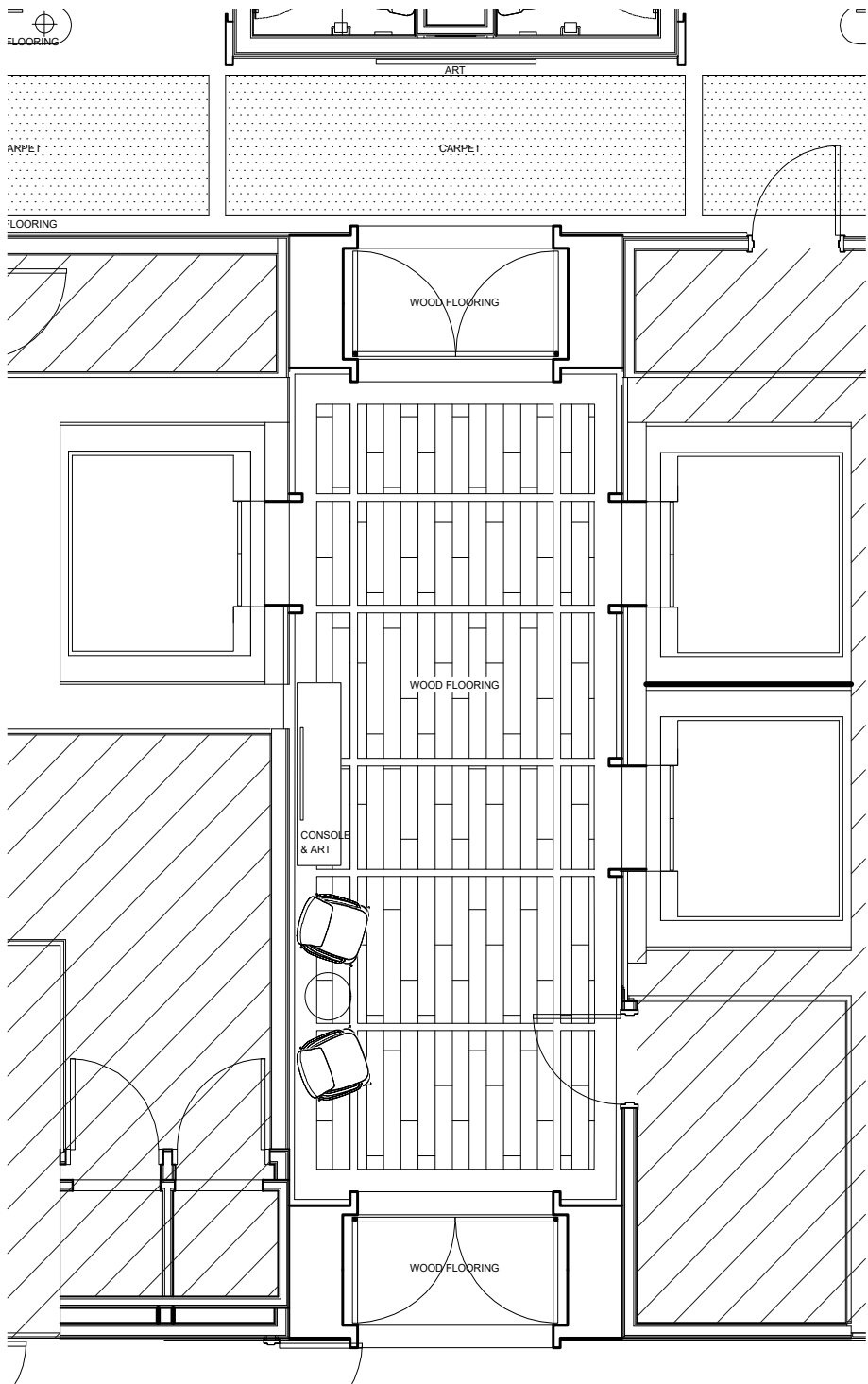
FLOOR PLAN
