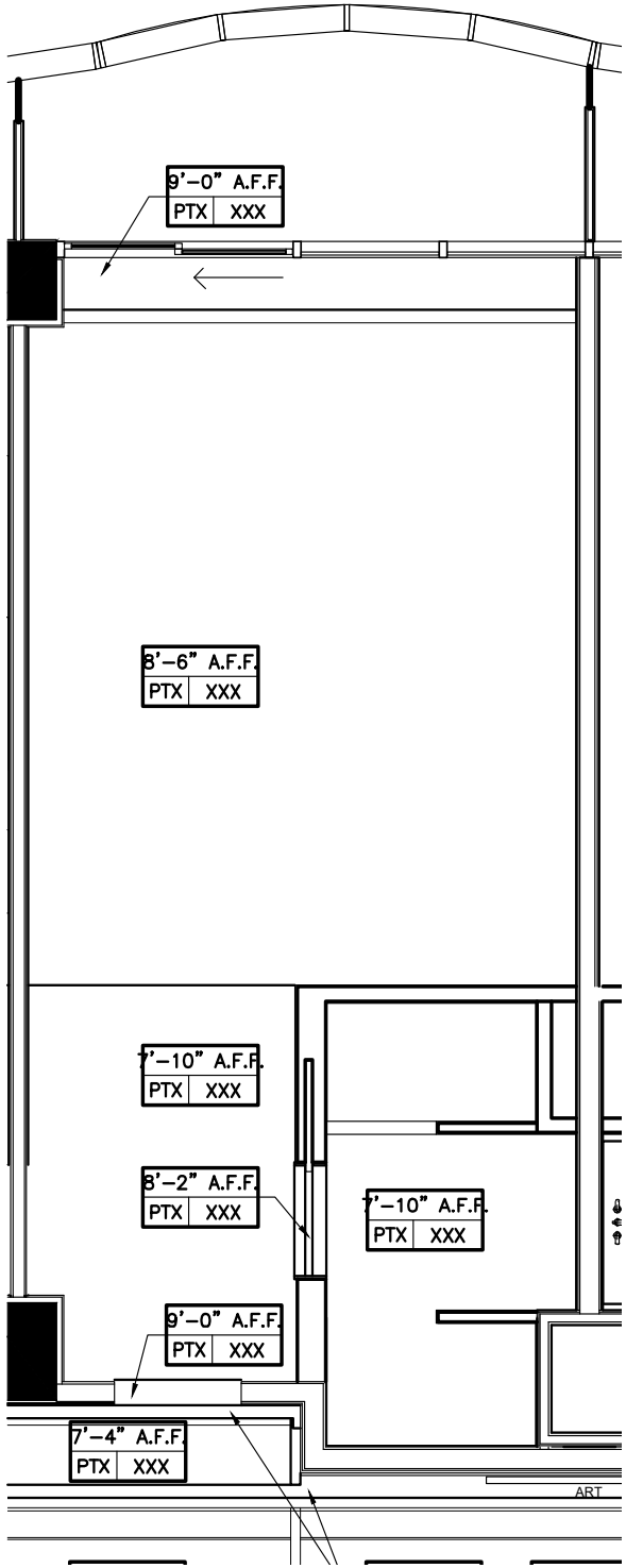
REFLECTED CEILING PLAN
