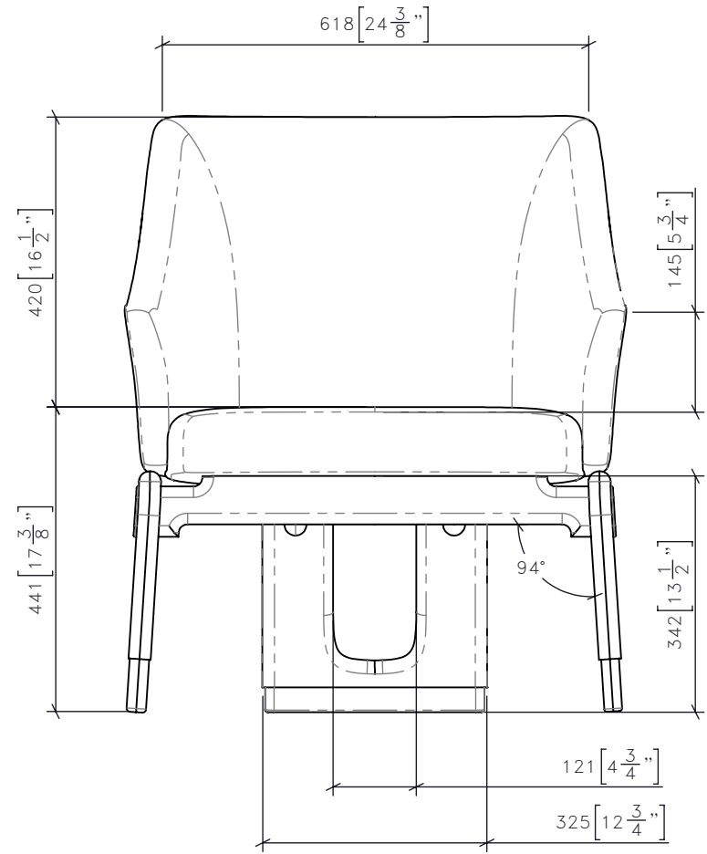
1 | SG-XX | 1:10 | VIP GUEST CHAIR FRONT ELEVATION
