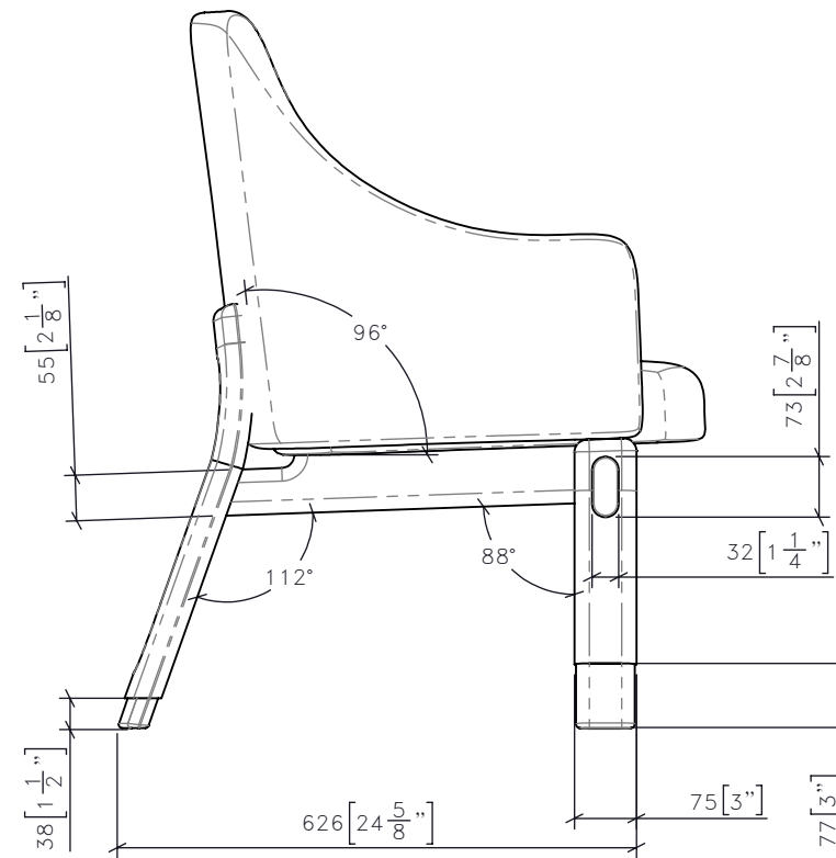
3 | SG-XX | 1:10 | VIP GUEST CHAIR SIDE ELEVATION
