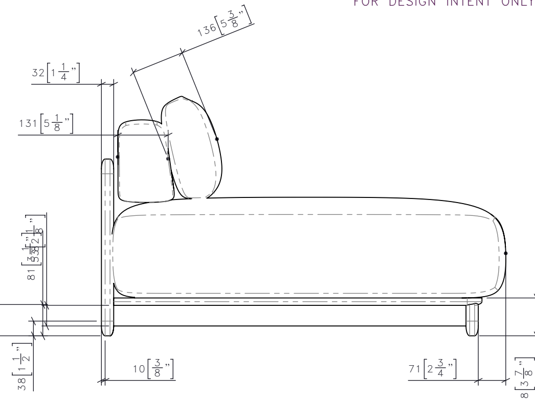
3 L2-SG-05 DAYBED SMALL (POOL) 1:10 SIDE ELEVATION
