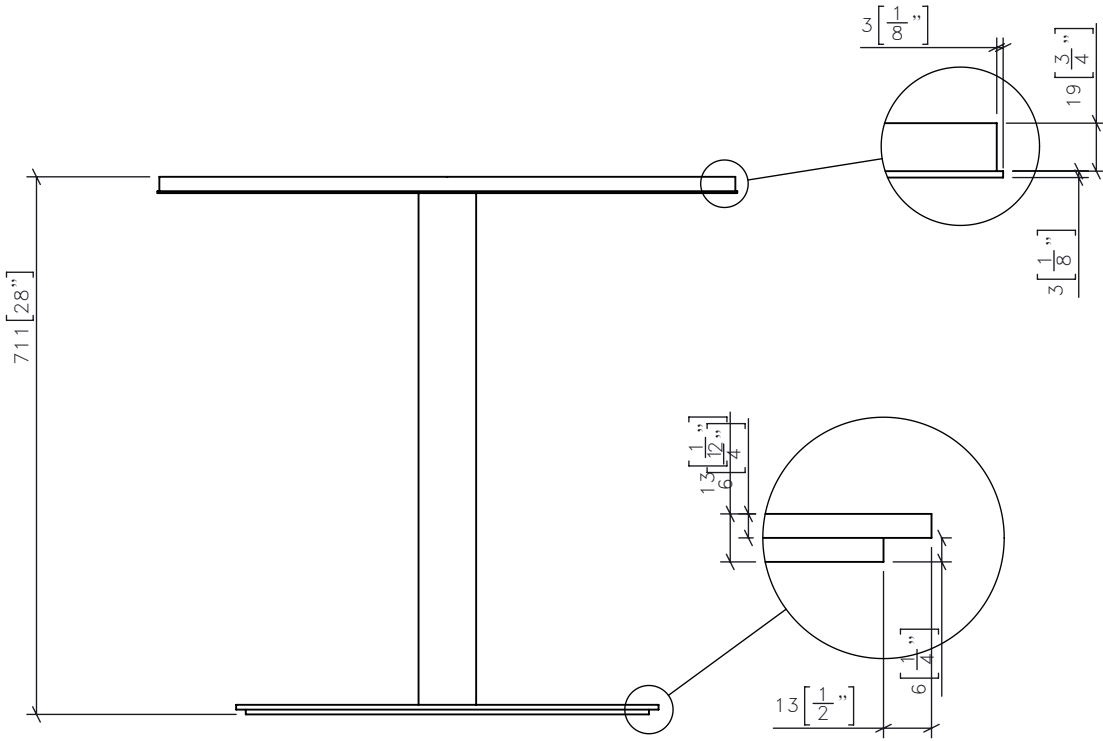
1 CG-05 1:10 ROUND DINING TABLE FRONT ELEVATION
