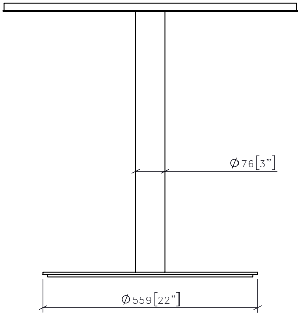
3 CG-05 1:10 ROUND DINING TABLE SIDE ELEVATION
