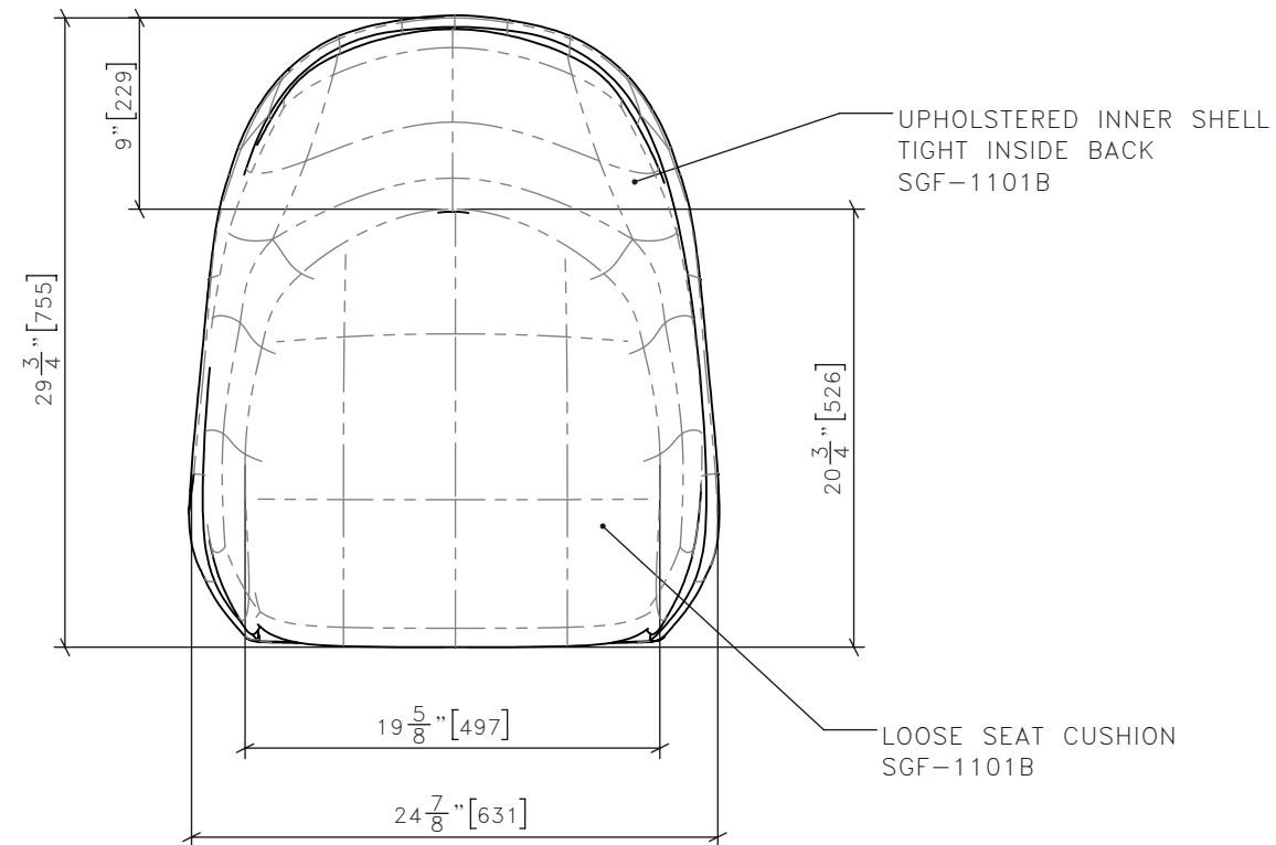
1 SG-1101 LOUNGE DINING CHAIR PLAN VIEW 1:8
