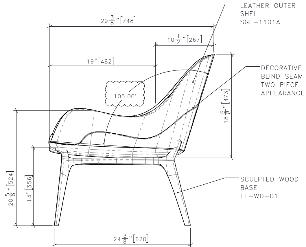
3 SG-1101 LOUNGE DINING CHAIR SIDE VIEW 1:8
