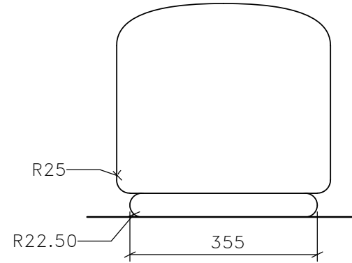
2 | SG-22 | OTTOMAN 2 1:10 | SIDE ELEVATION
