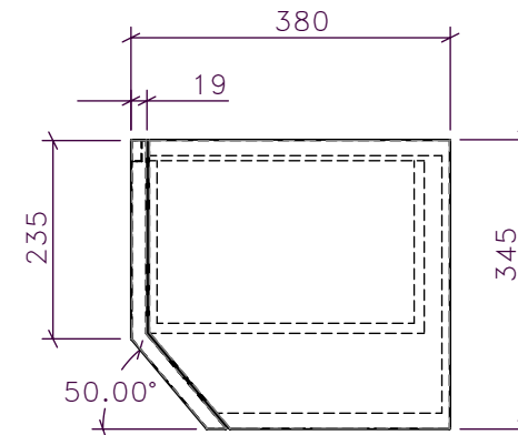
3 CG-XX TV CABINET 1:10 SIDE ELEVATION
