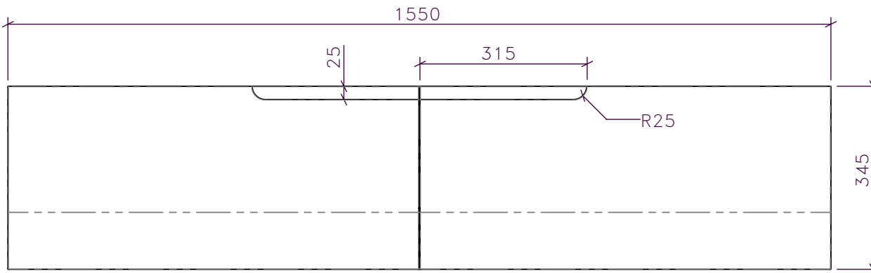
1 CG-XX TV CABINET 1:10 FRONT ELEVATION
