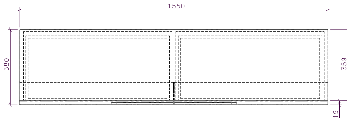
2 CG-XX TV CABINET 1:10 PLAN
