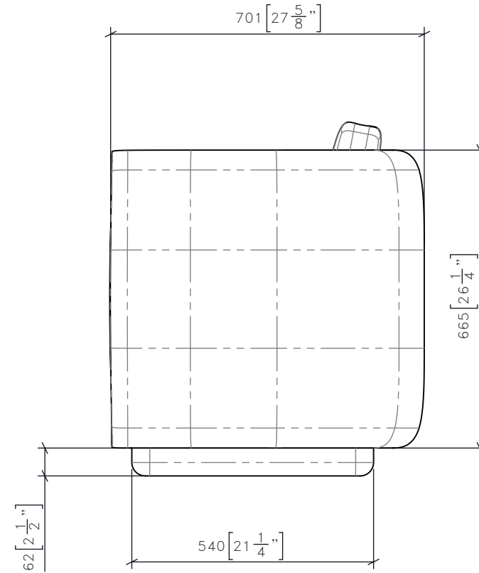
1 | SG-XX 1:12 | SOFA SIDE VIEW
