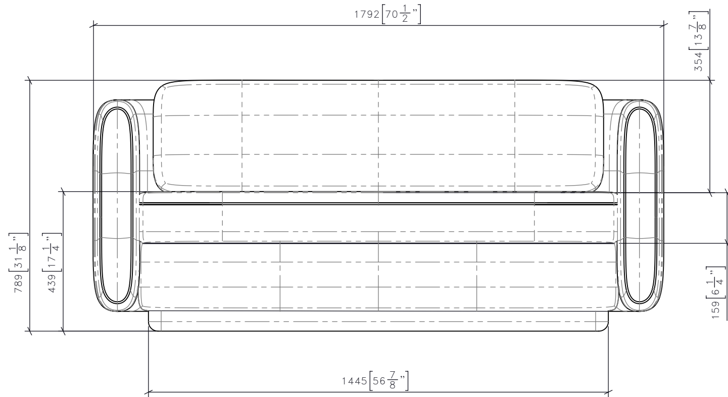
1 | SG-XX 1:12 | SOFA FRONT VIEW
