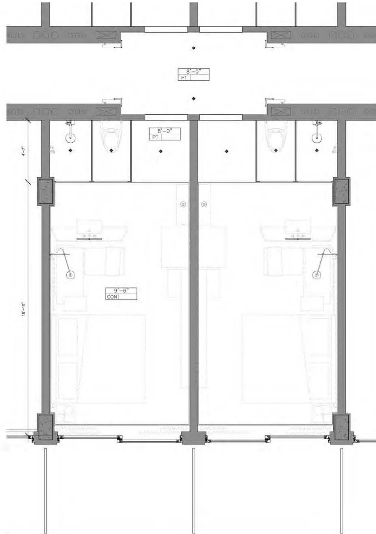
TYPICAL GUESTROOM (OPTION 2) - REFLECTED CEILING PLAN
