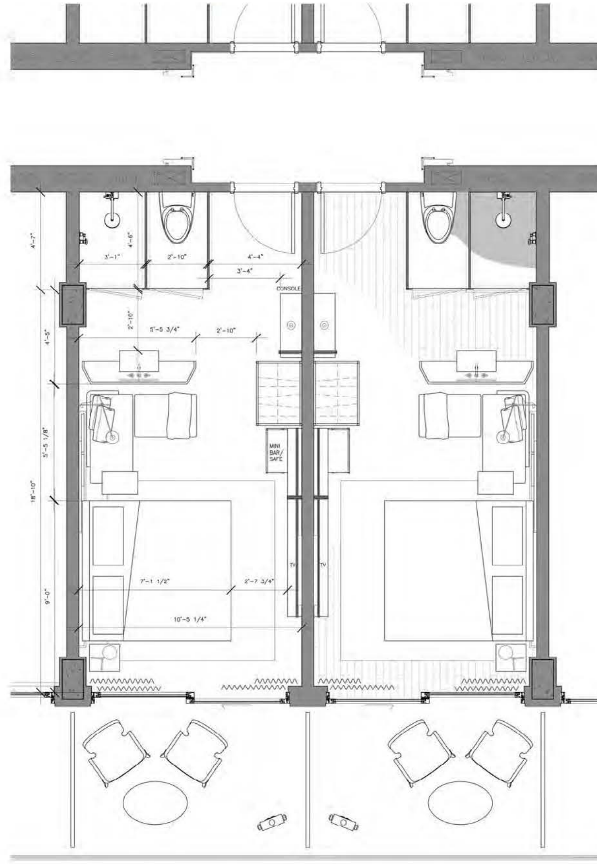
TYPICAL GUESTROOM (OPTION 2) - FLOOR PLAN
