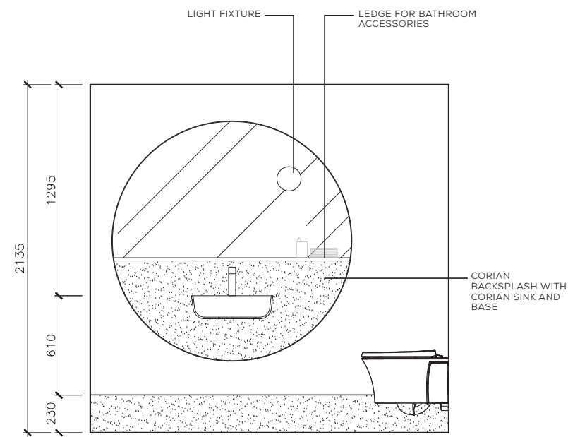
2 TYPICAL WASHROOM ELEVATION N.T.S.
