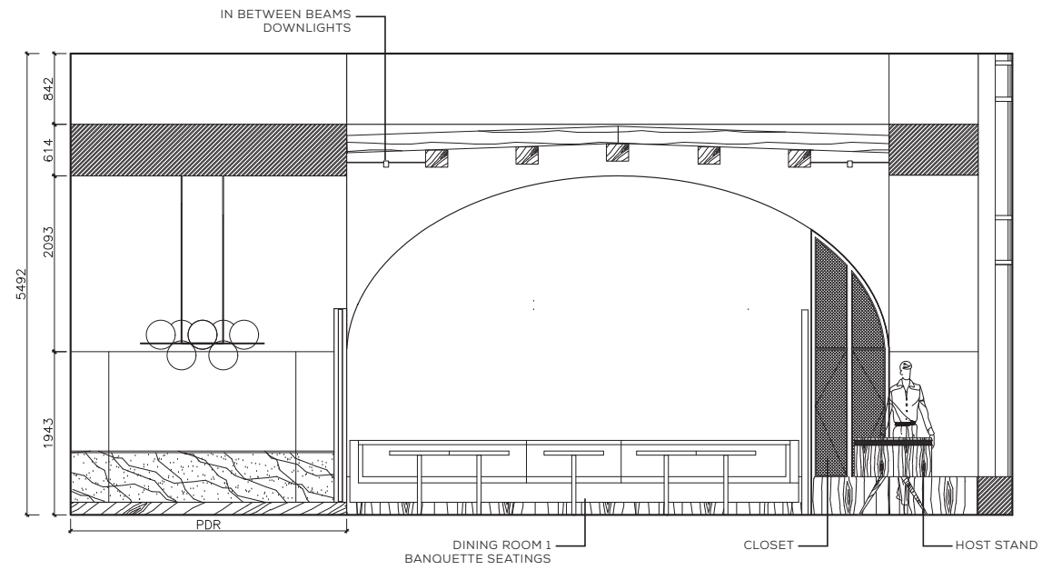
2 DINING ROOM EAST ELEVATION N.T.S.
