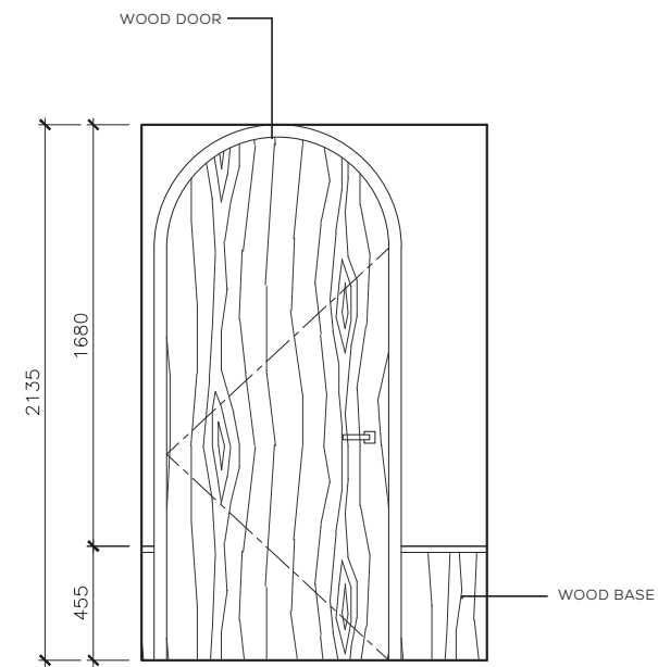
1 BASEMENT MEZZANINE WASHROOM CORRIDOR ELEVATION N.T.S.
