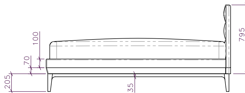
4 CG-XX 1:25 DARK SCHEME QUEEN BED 02 SIDE ELEVATION
