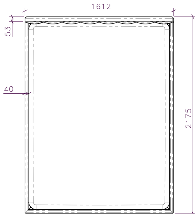
1 CG-XX 1:25 DARK SCHEME QUEEN BED 02 PLAN
