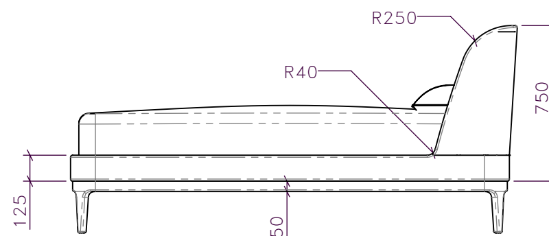
4 CG-XX 1:25 DARK SCHEME QUEEN BED 01 SIDE ELEVATION
