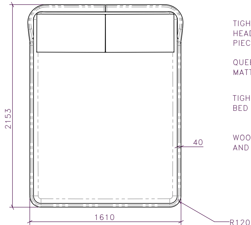
1 CG-XX 1:25 DARK SCHEME QUEEN BED 01 PLAN
