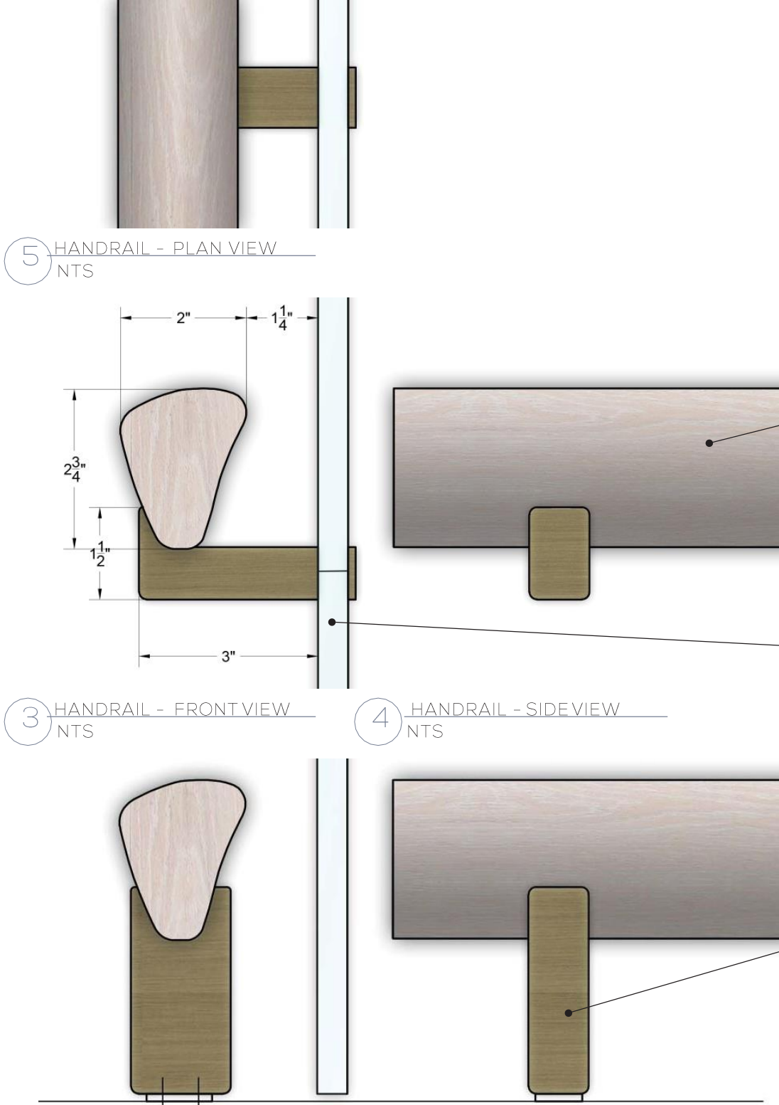
1 HANDRAIL - FRONT VIEW NTS
