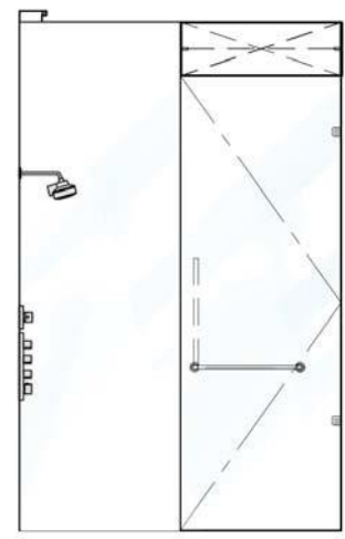
6 MASTER SHOWER NORTH ELEVATION NTS
