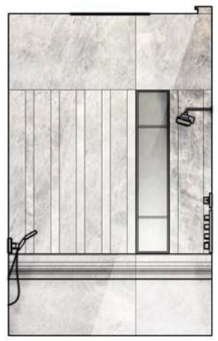
4 MASTER SHOWER SOUTH ELEVATION NTS
