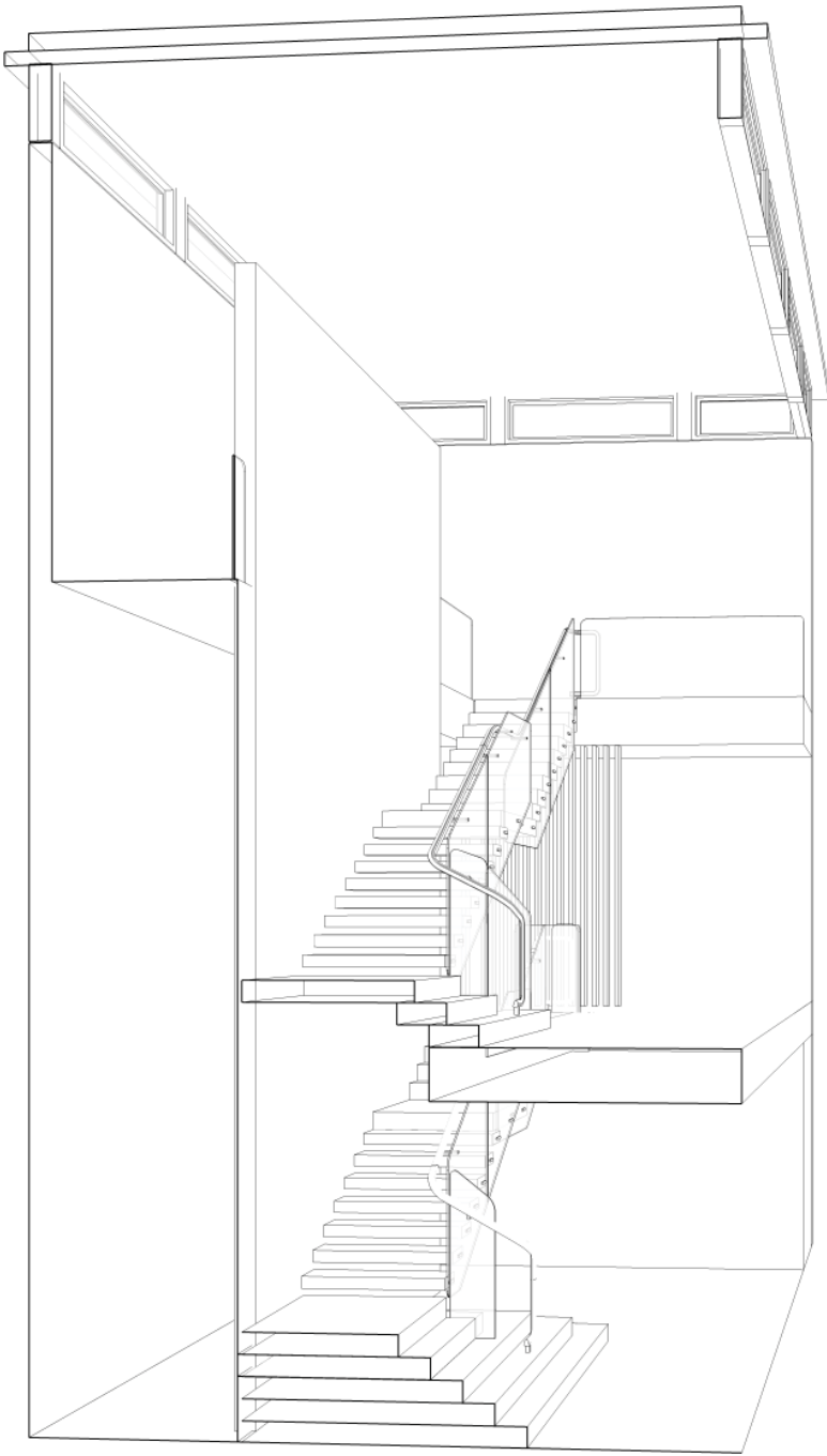
1 3D SKETCH UP VIEW - STAIRCASE SECTION NTS
