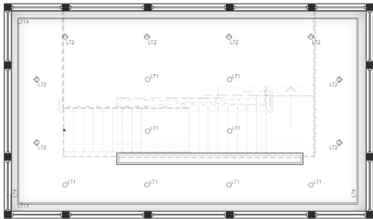
4 CUPOLA REFLECTED CEILING PLAN NTS
