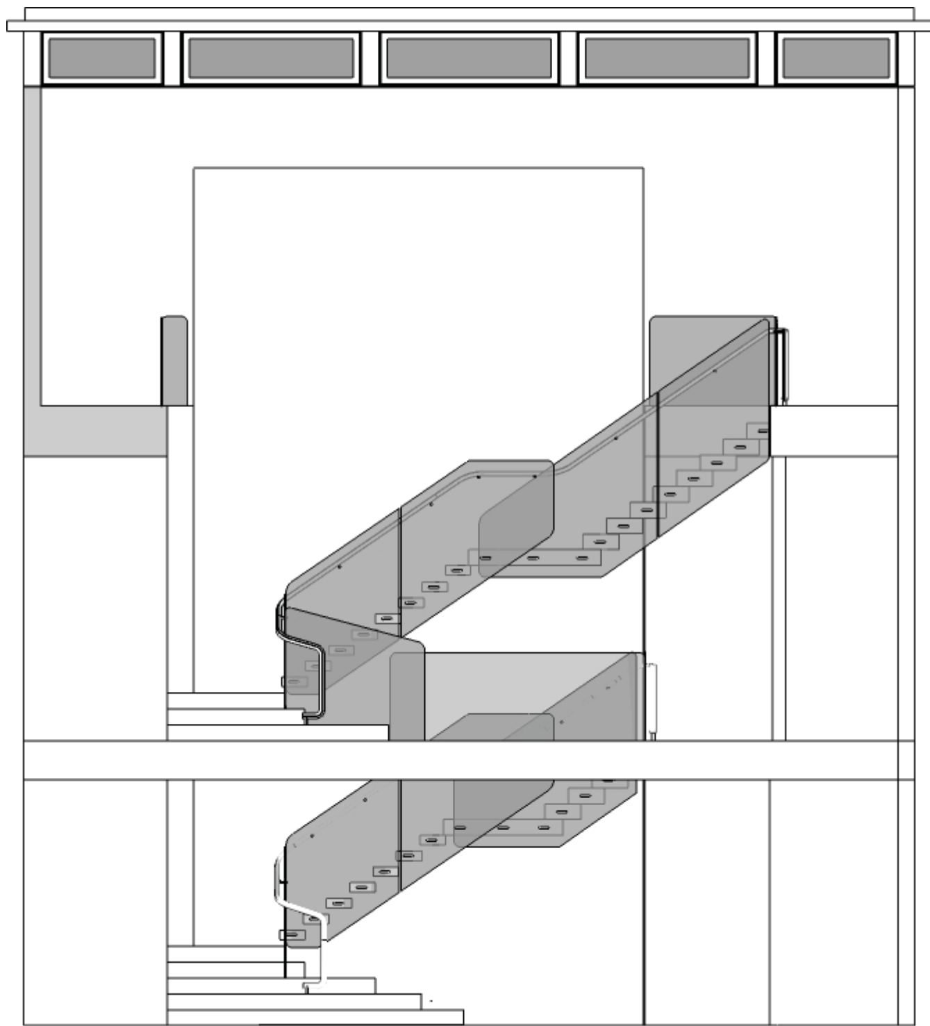
6 SECTION VIEW NTS
