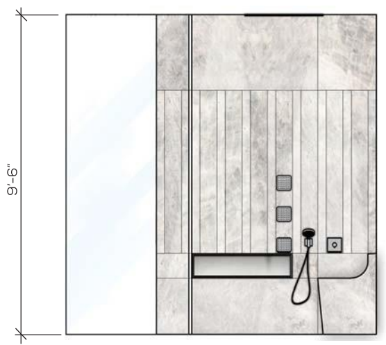
3 MASTER SHOWER EAST ELEVATION NTS
