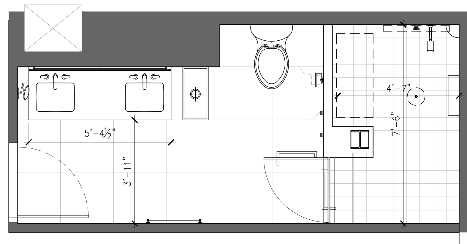
SECOND FLOOR
