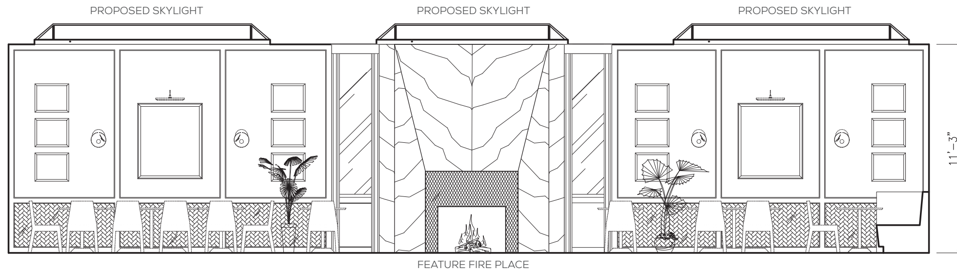
2 DINING ROOM WEST ELEVATION
