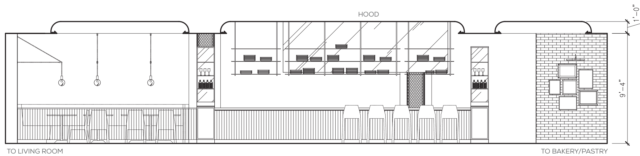
2 KITCHEN EAST ELEVATION
