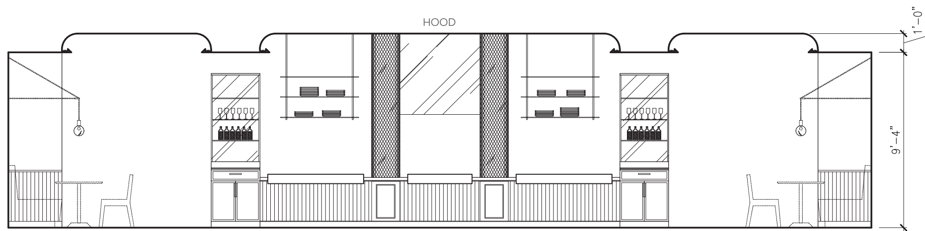
1 KITCHEN SOUTH ELEVATION
