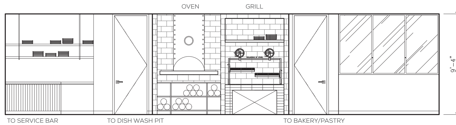
1 KITCHEN OVEN AND GRILL ELEVATION
