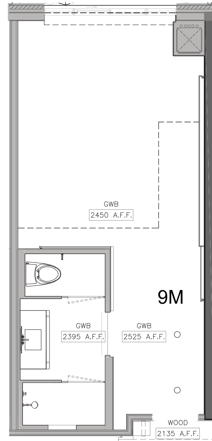
REFLECTIVE CEILING PLAN
