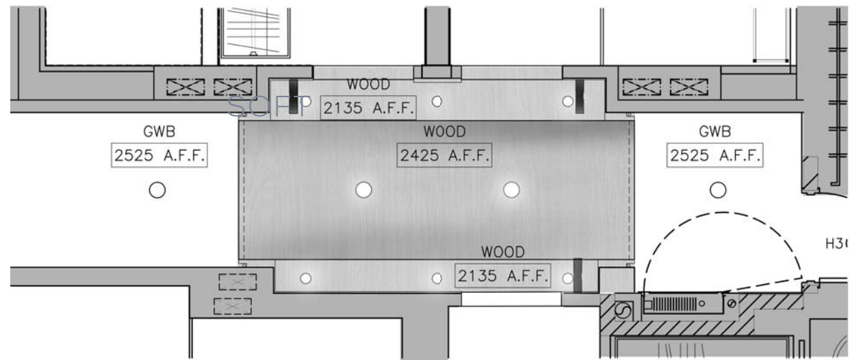
CORRIDOR REFLECTIVE CEILING PLAN
