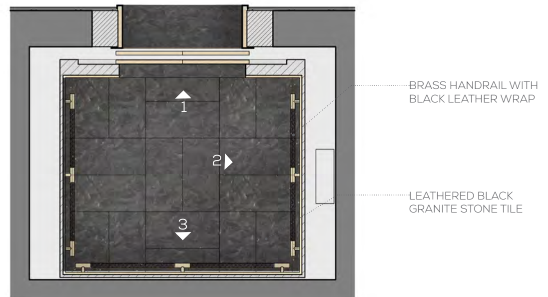
5 ENLARGED ELEVATOR CAB PLAN NTS
