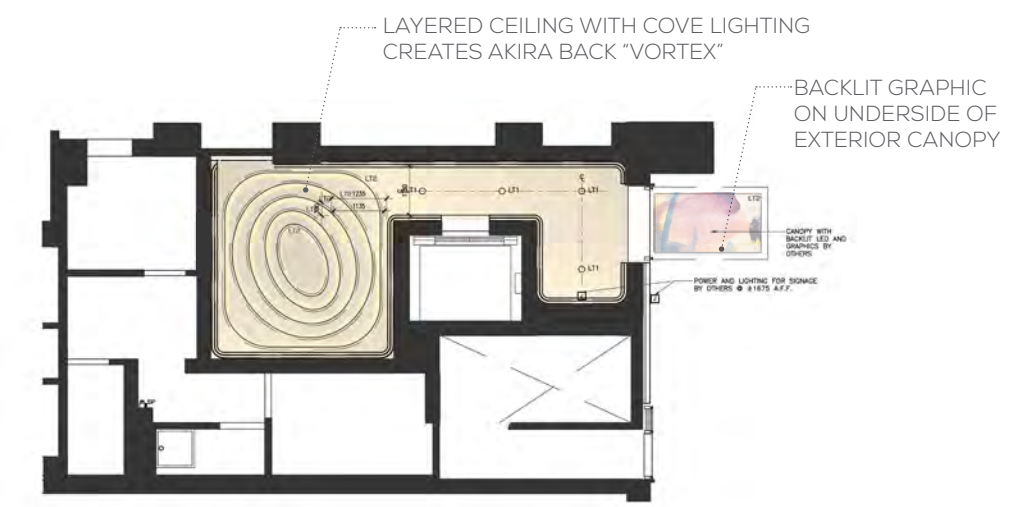
2 GROUND FLOOR CEILING PLAN NTS
