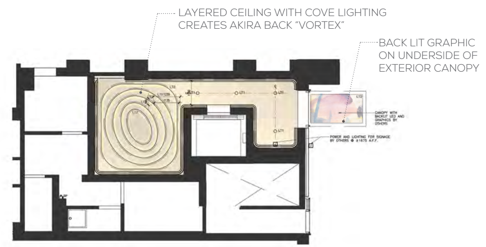
2 GROUND FLOOR CEILING PLAN NTS
