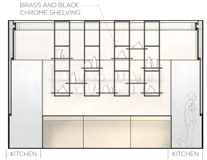
3 SUSHI BAR ELEVATION NTS
