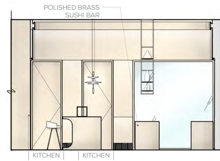
4 SECTION THROUGH SUSHI BAR NTS
