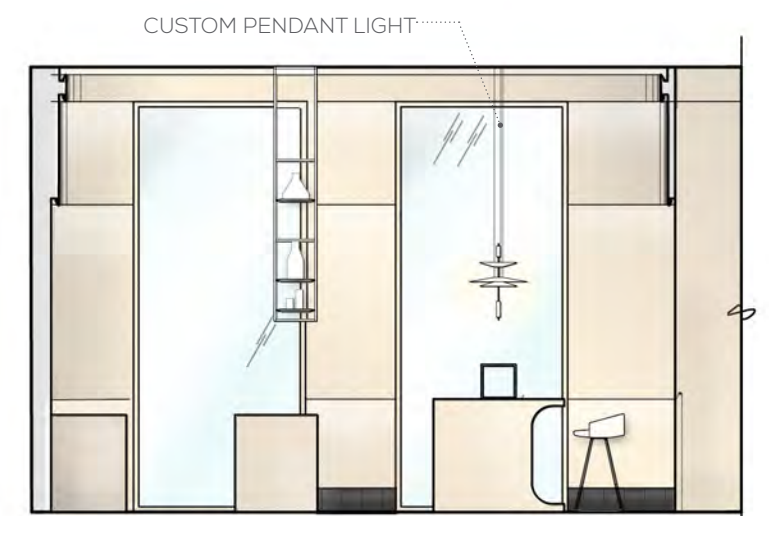
6 SECTION THROUGH SUSHI BAR NTS
