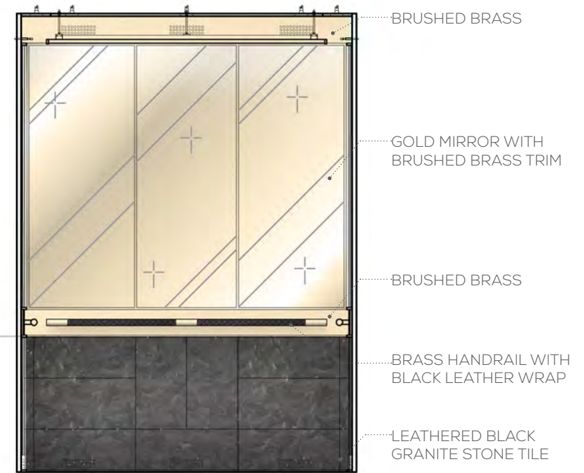
3 ELEVATOR CAB ELEVATION NTS
