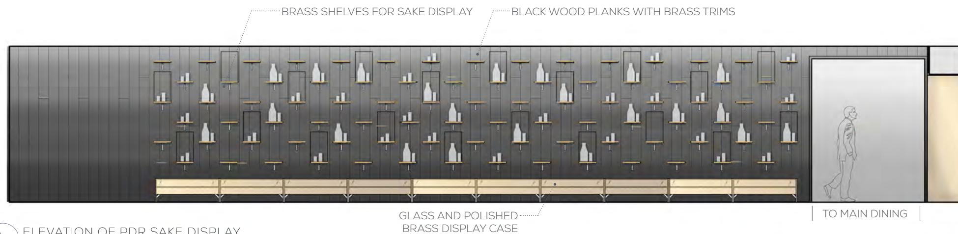
1 ELEVATION OF PDR SAKE DISPLAY NTS
