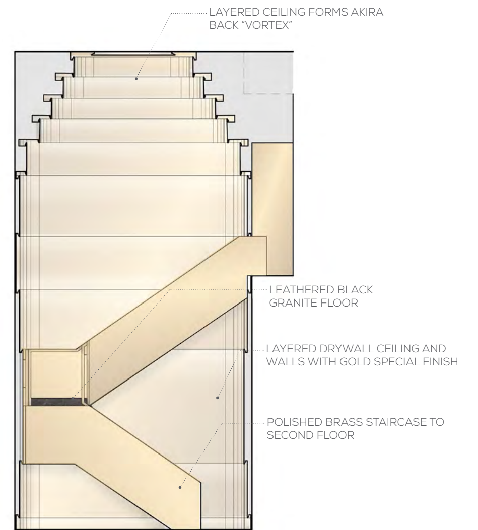
3 SECTION THROUGH STAIRS NTS
