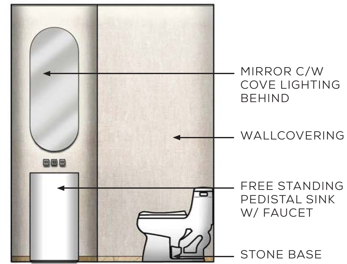
NORTH ELEVATION
