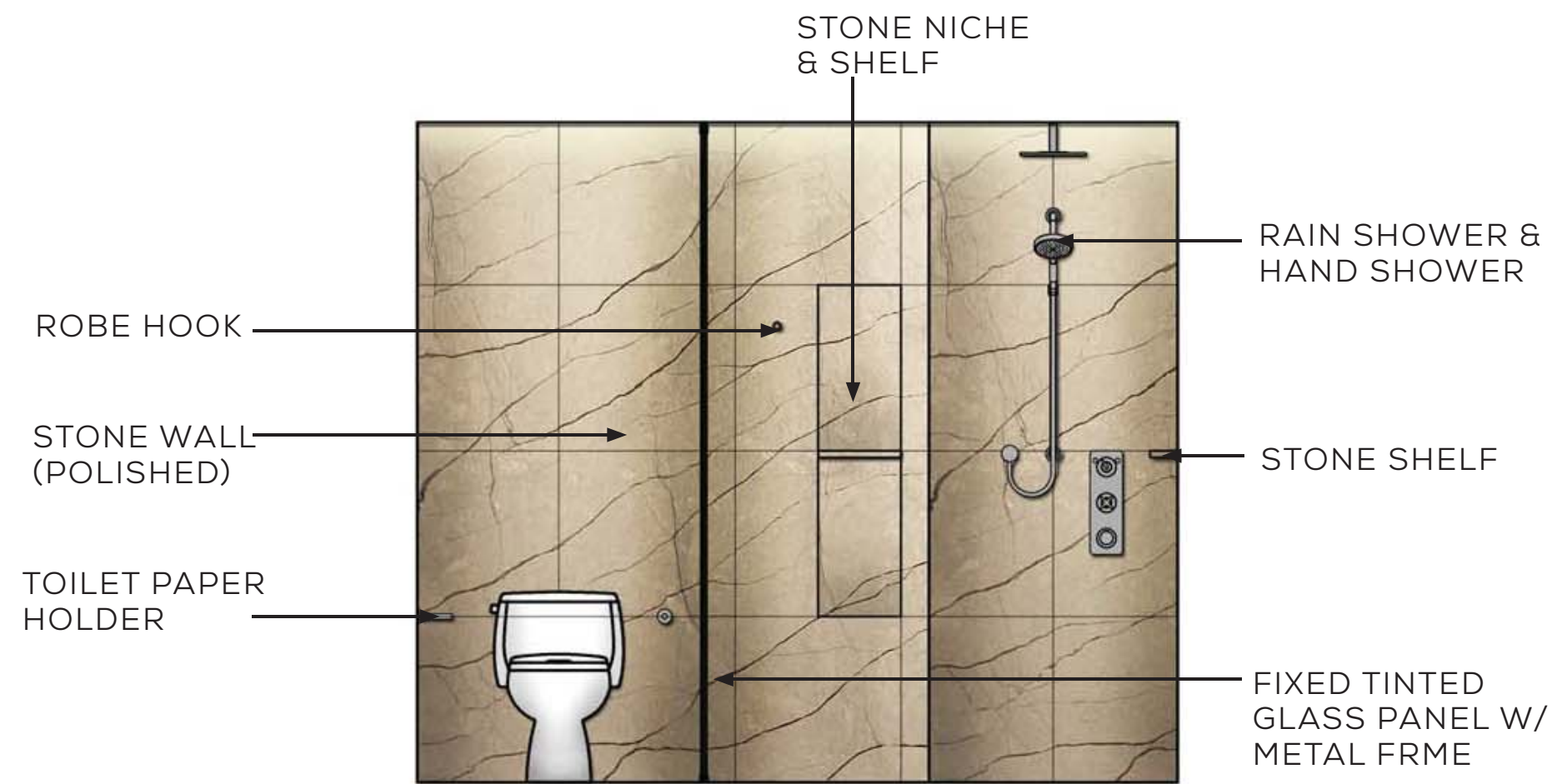
WEST ELEVATION
