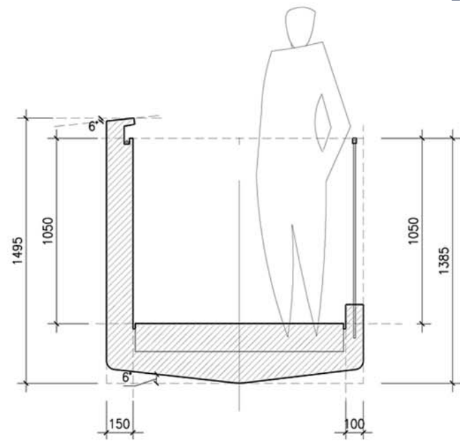
RAILING PROFILE OPTION 1
