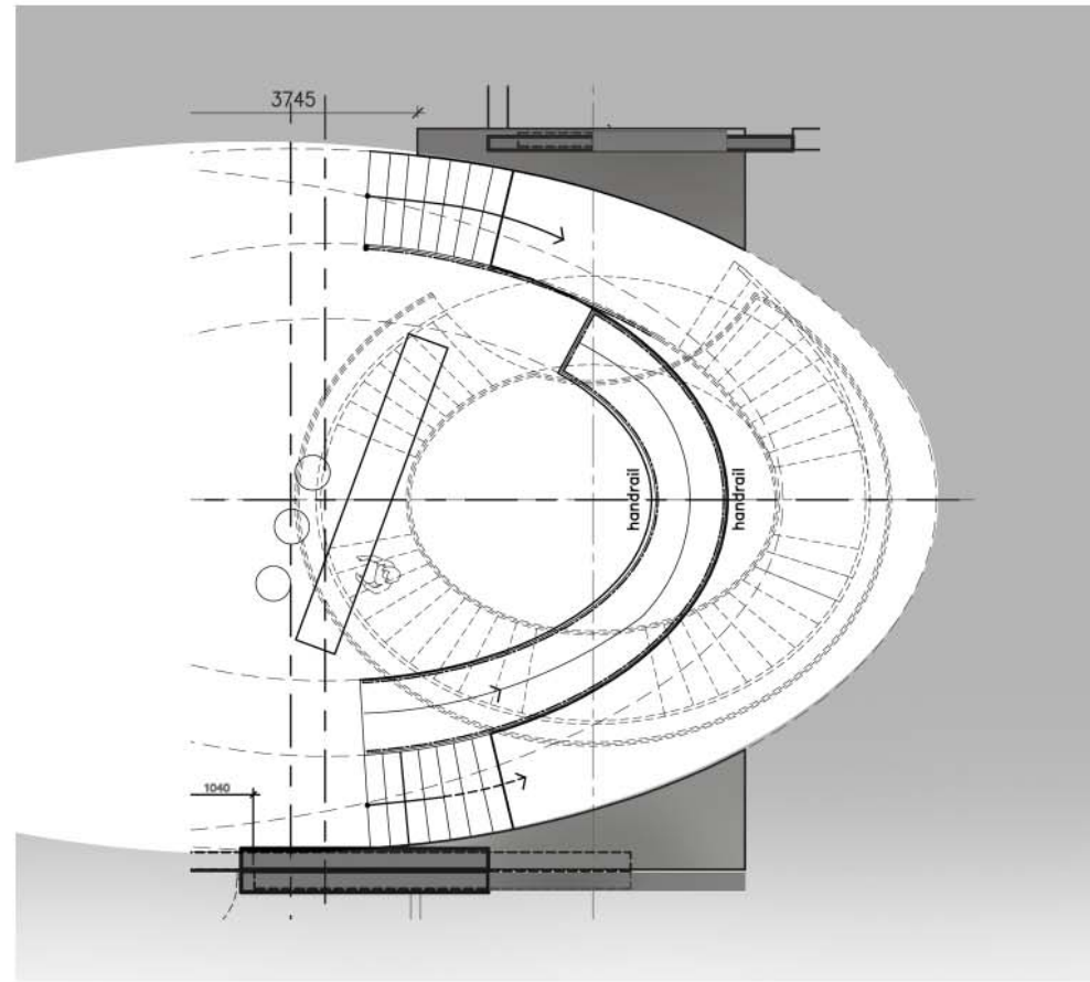
LOWER TO GROUND FLOOR
