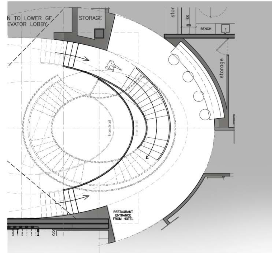
GROUND FLOOR TO 2ND FLOOR
