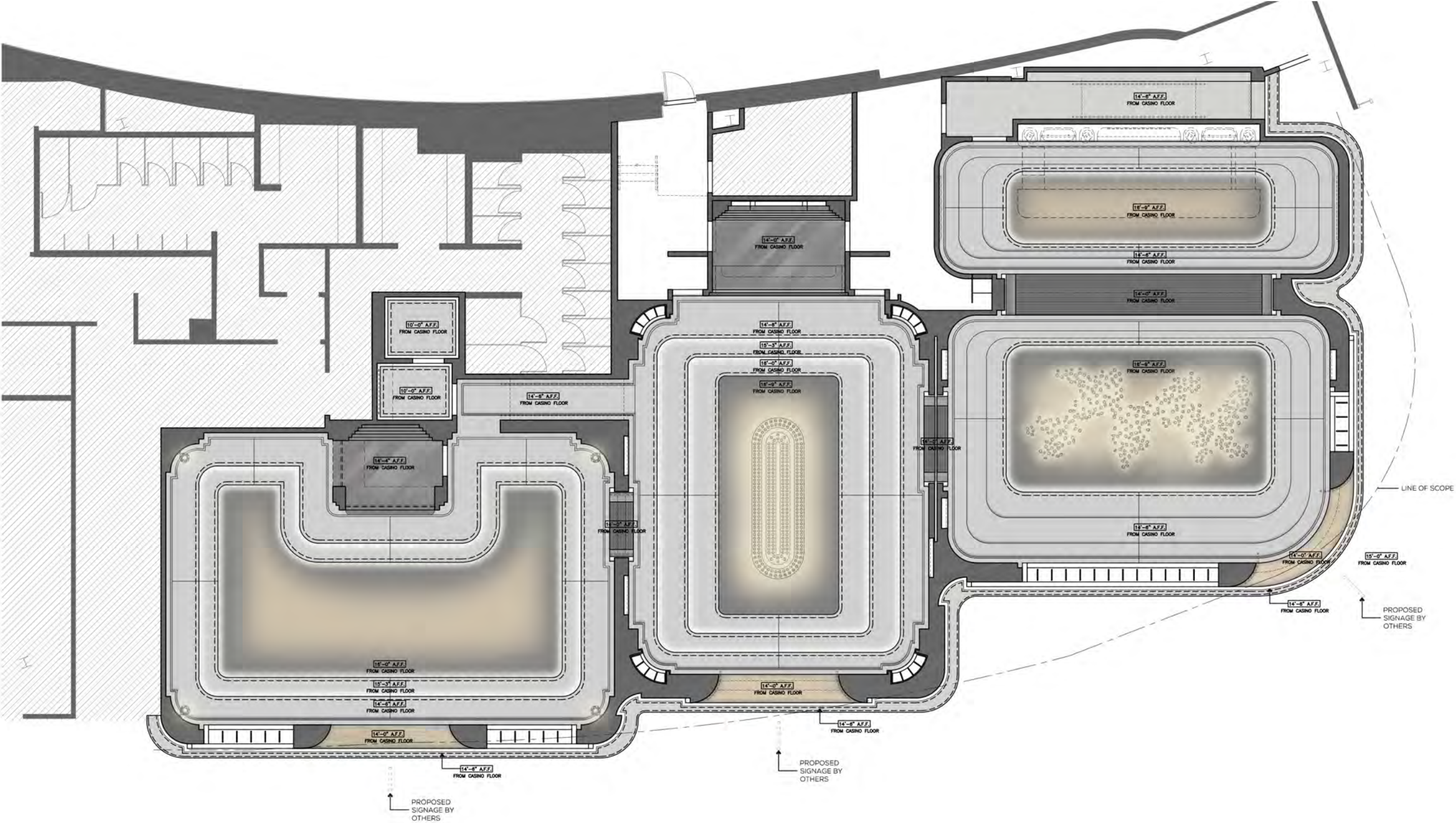
1 REFLECTED CEILING PLAN NTS
